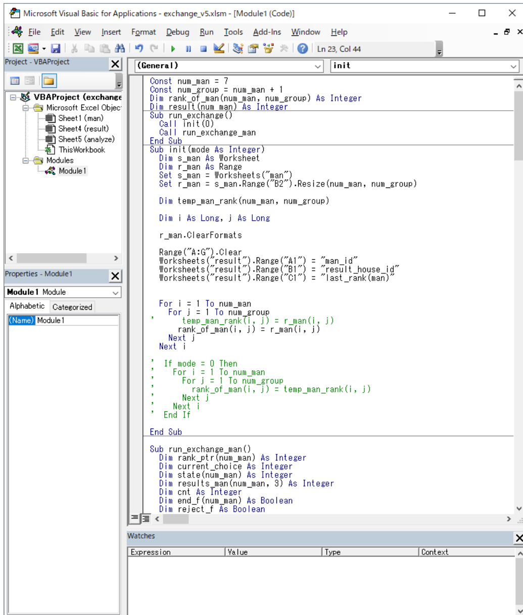
Figure 4: VBA window
